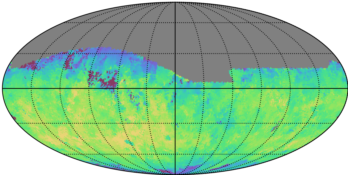
baseline_v3.5_10yrs Yr 1 r band: Median fiveSigmaDepth
