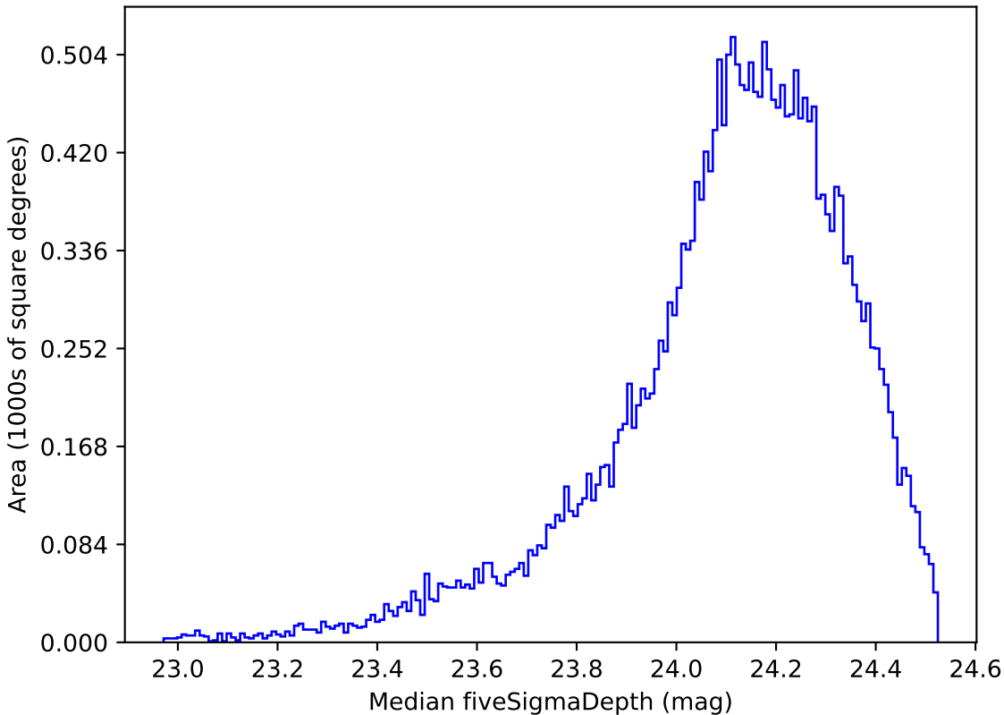
baseline_v3.5_10yrs Yr 1 r band: Median fiveSigmaDepth
