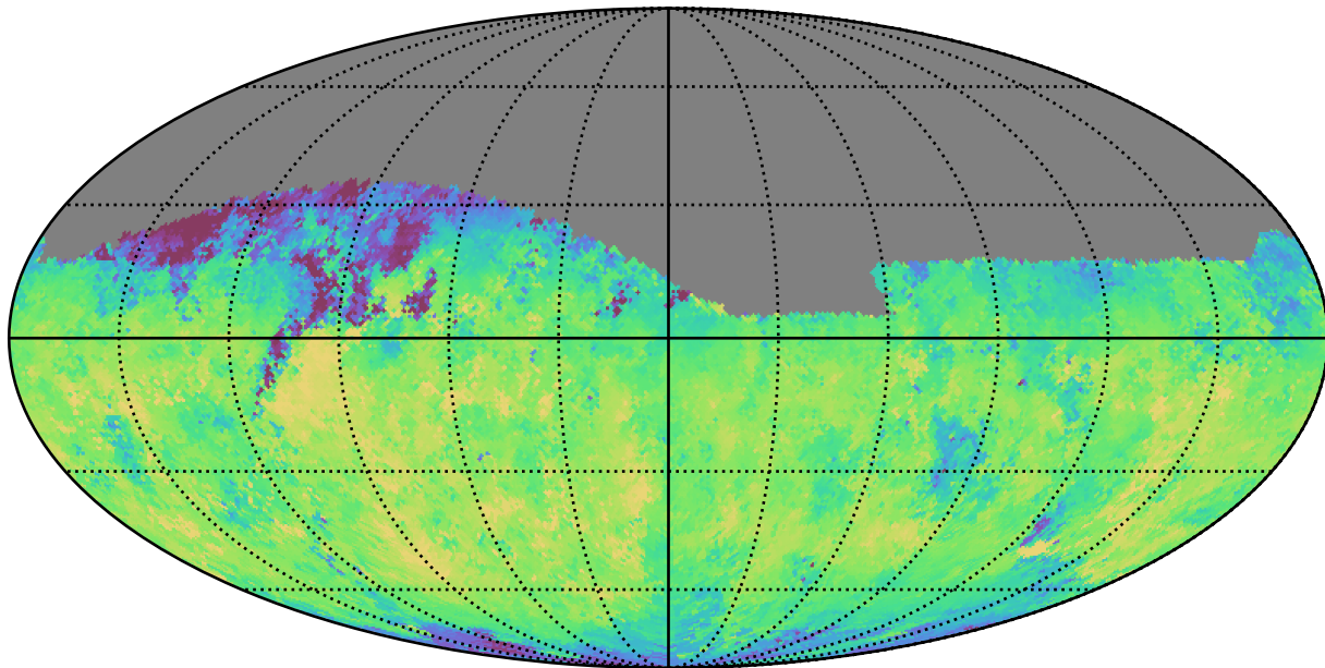
baseline_v3.5_10yrs Yr 1 i band: Median fiveSigmaDepth
