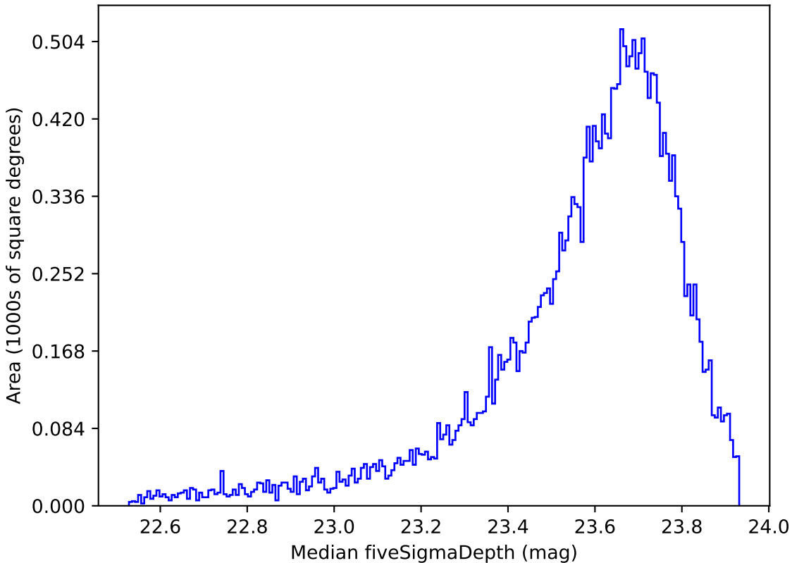
baseline_v3.5_10yrs Yr 1 i band: Median fiveSigmaDepth
