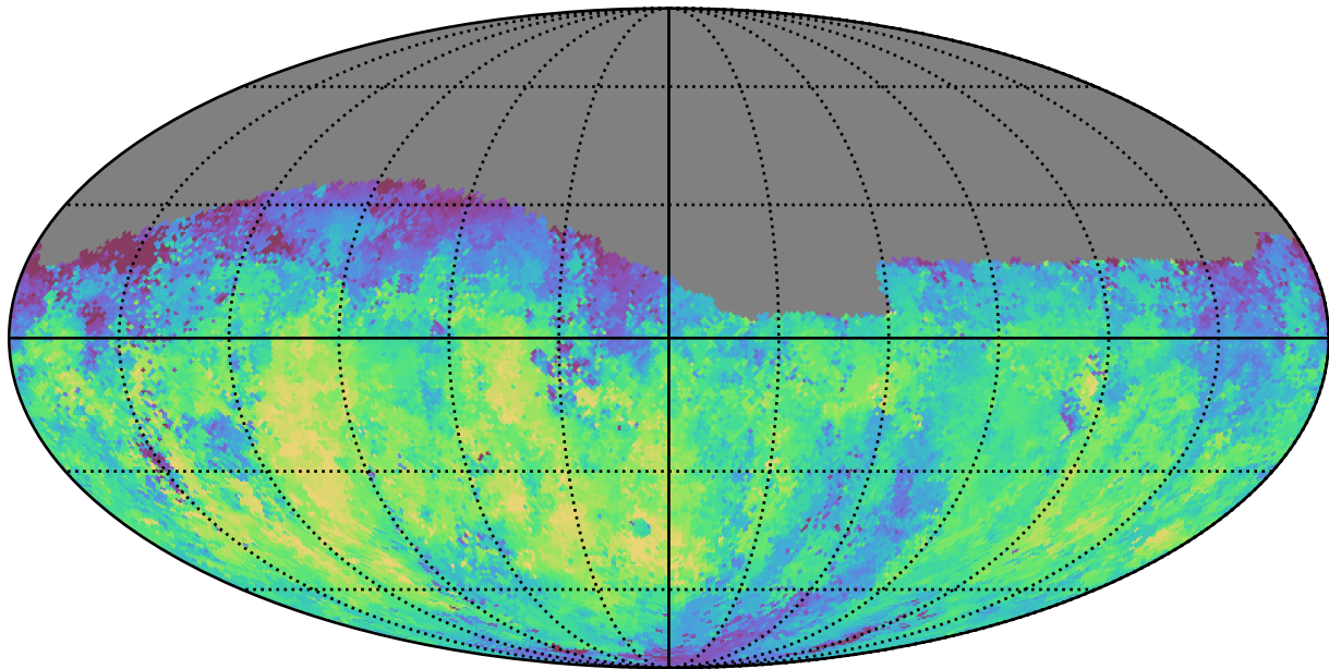
baseline_v3.5_10yrs Yr 1 g band: Median fiveSigmaDepth
