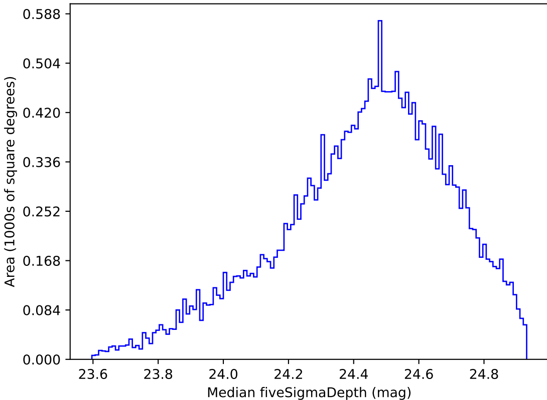
baseline_v3.5_10yrs Yr 1 g band: Median fiveSigmaDepth
