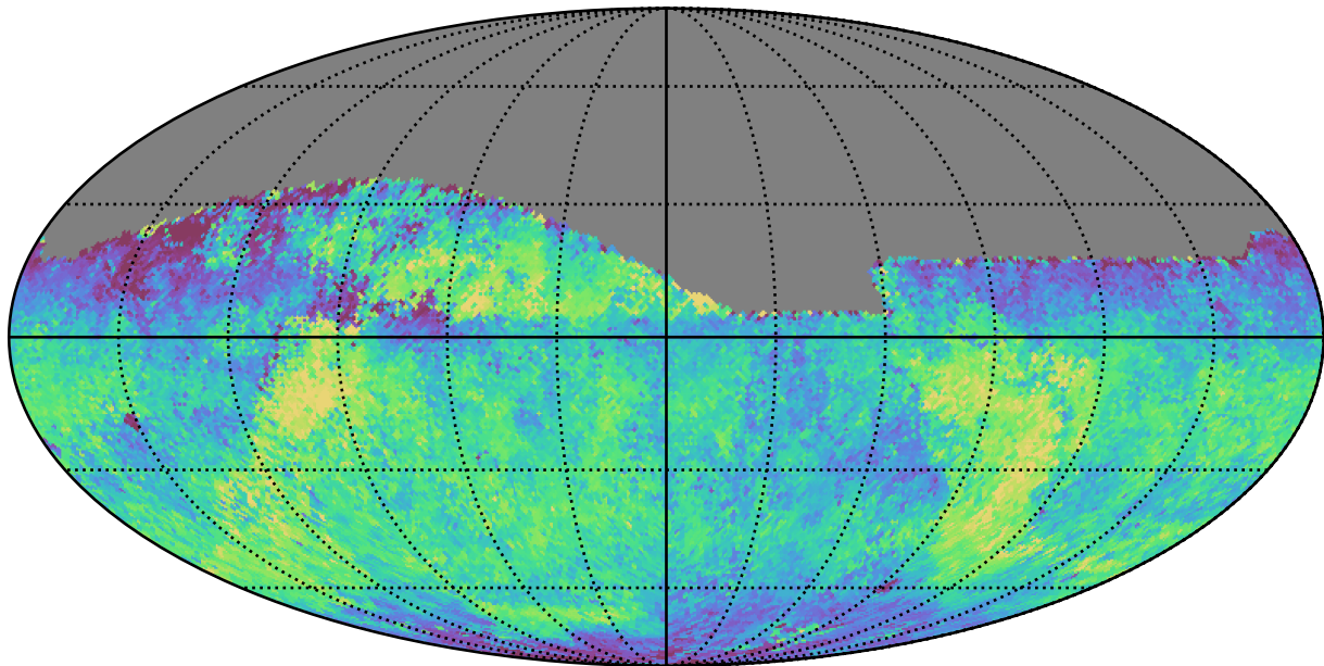
baseline_v3.5_10yrs Yr 1 all bands: Median fiveSigmaDepth
