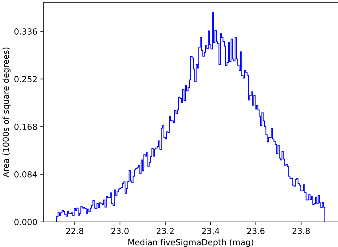
baseline_v3.5_10yrs Yr 1 all bands: Median fiveSigmaDepth
