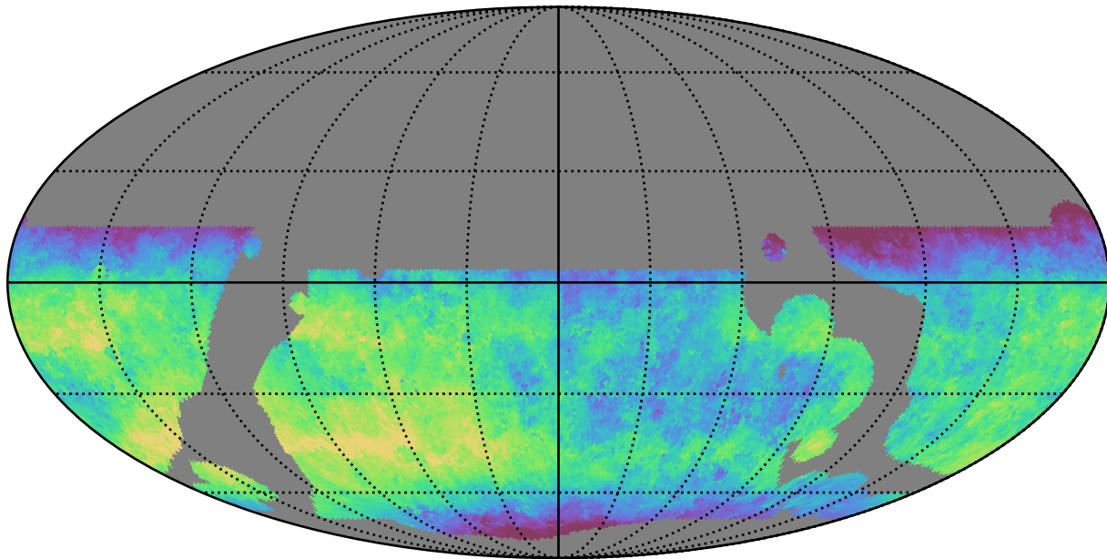
baseline_v3.5_10yrs WFD z band: Median fiveSigmaDepth
