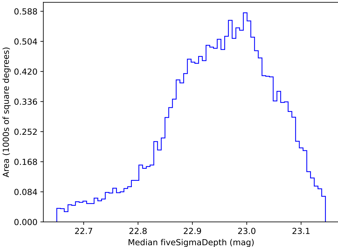
baseline_v3.5_10yrs WFD z band: Median fiveSigmaDepth
