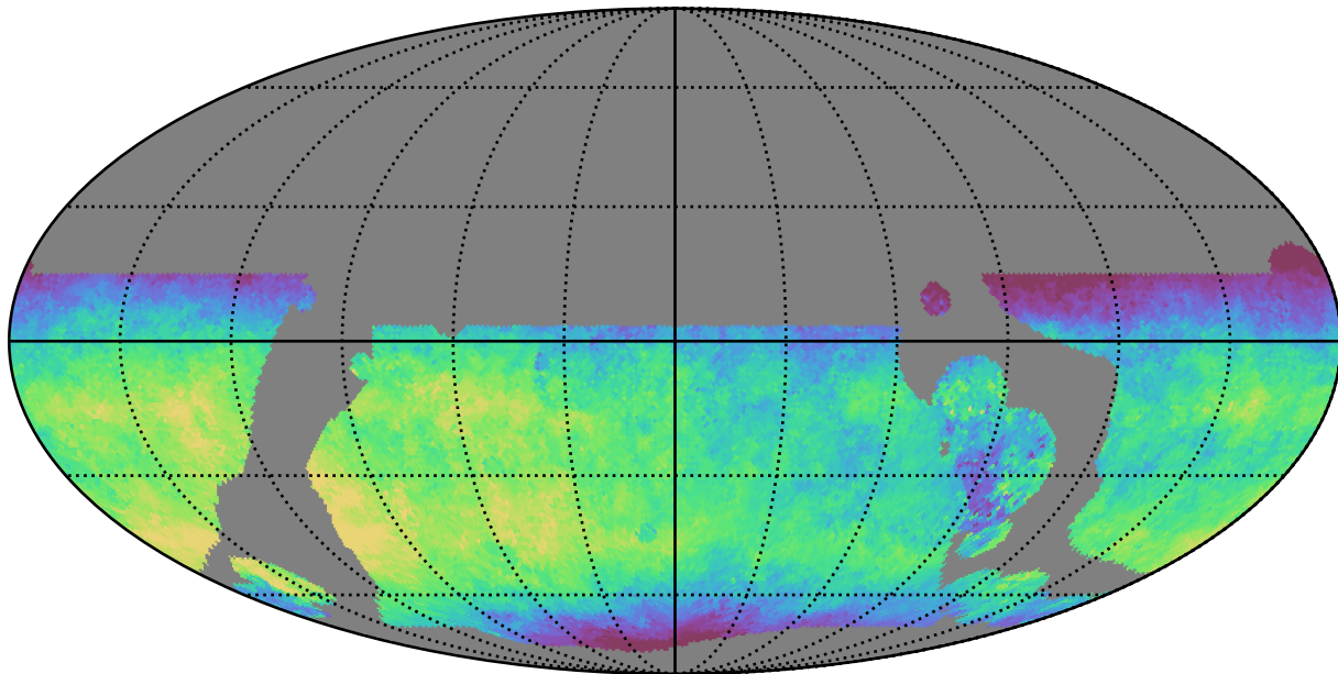
baseline_v3.5_10yrs WFD y band: Median fiveSigmaDepth
