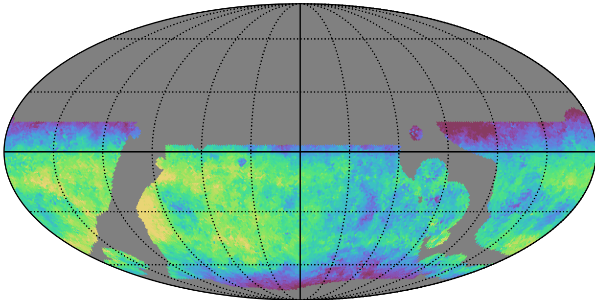
baseline_v3.5_10yrs WFD u band: Median fiveSigmaDepth
