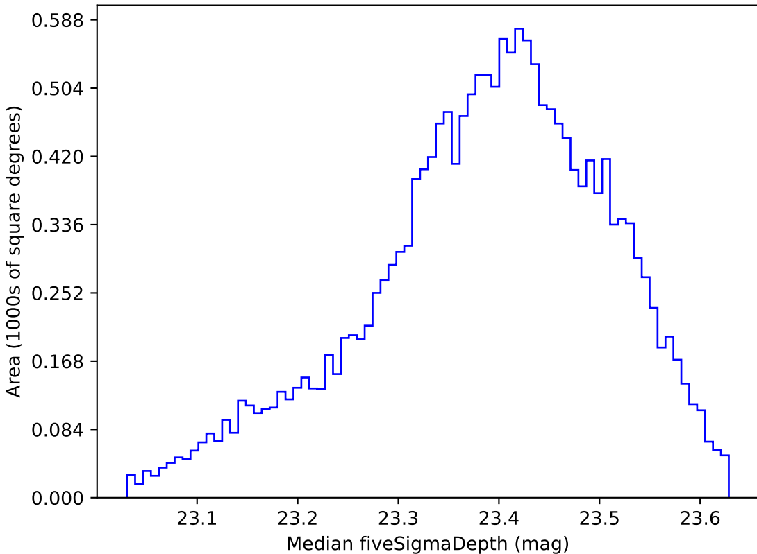
baseline_v3.5_10yrs WFD u band: Median fiveSigmaDepth
