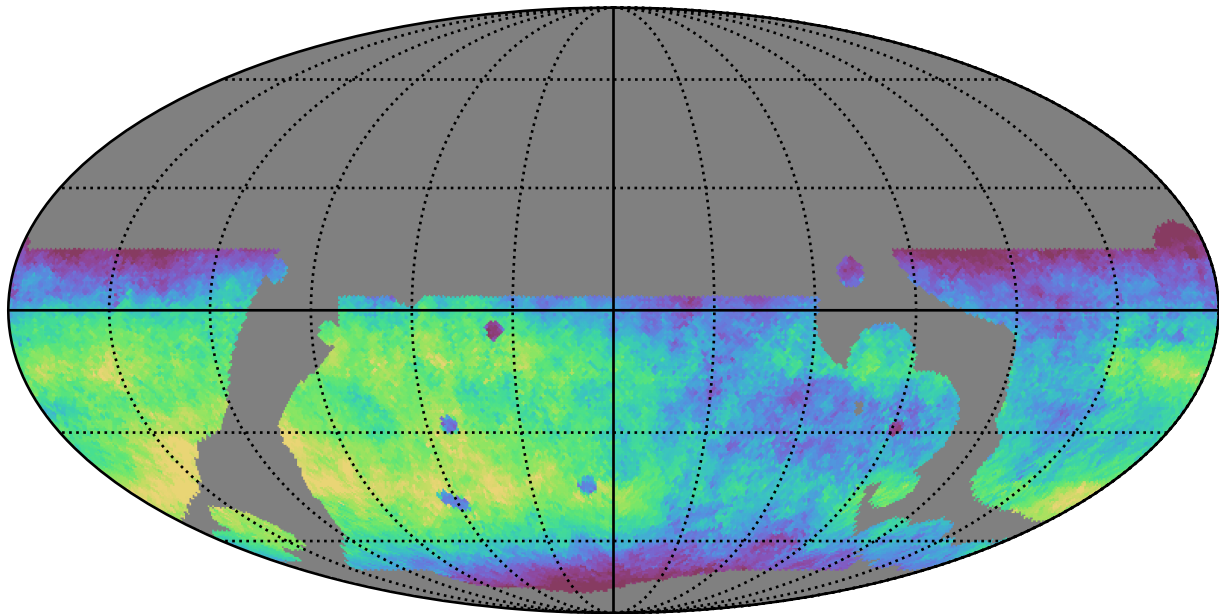
baseline_v3.5_10yrs WFD r band: Median fiveSigmaDepth
