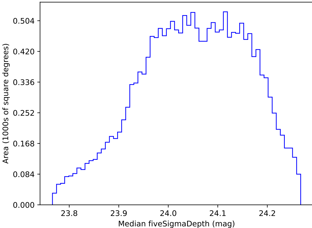
baseline_v3.5_10yrs WFD r band: Median fiveSigmaDepth
