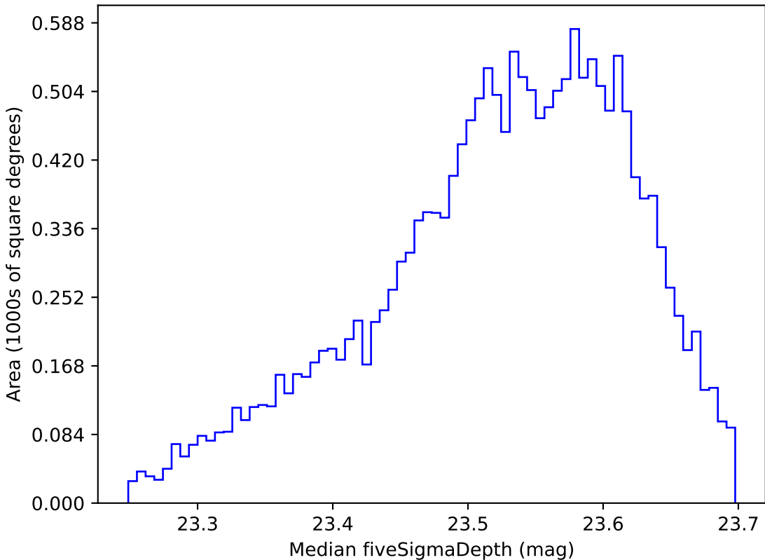
baseline_v3.5_10yrs WFD i band: Median fiveSigmaDepth
