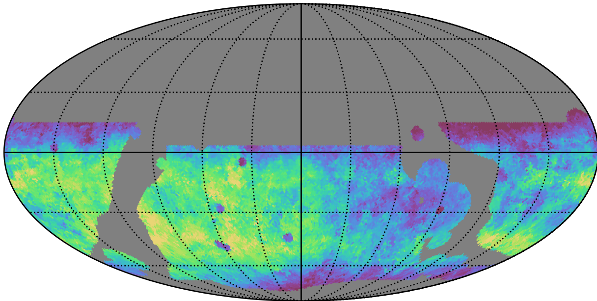
baseline_v3.5_10yrs WFD g band: Median fiveSigmaDepth
