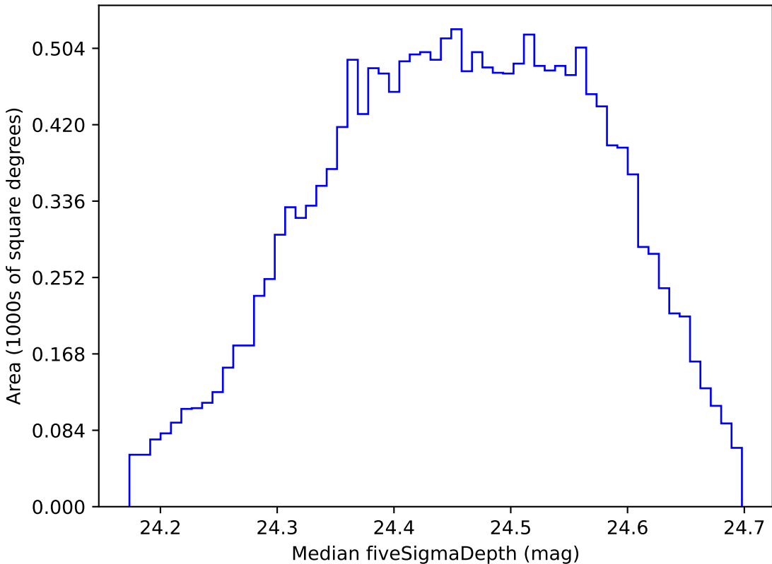
baseline_v3.5_10yrs WFD g band: Median fiveSigmaDepth
