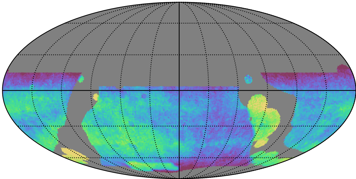
baseline_v3.5_10yrs WFD all bands: Median fiveSigmaDepth
