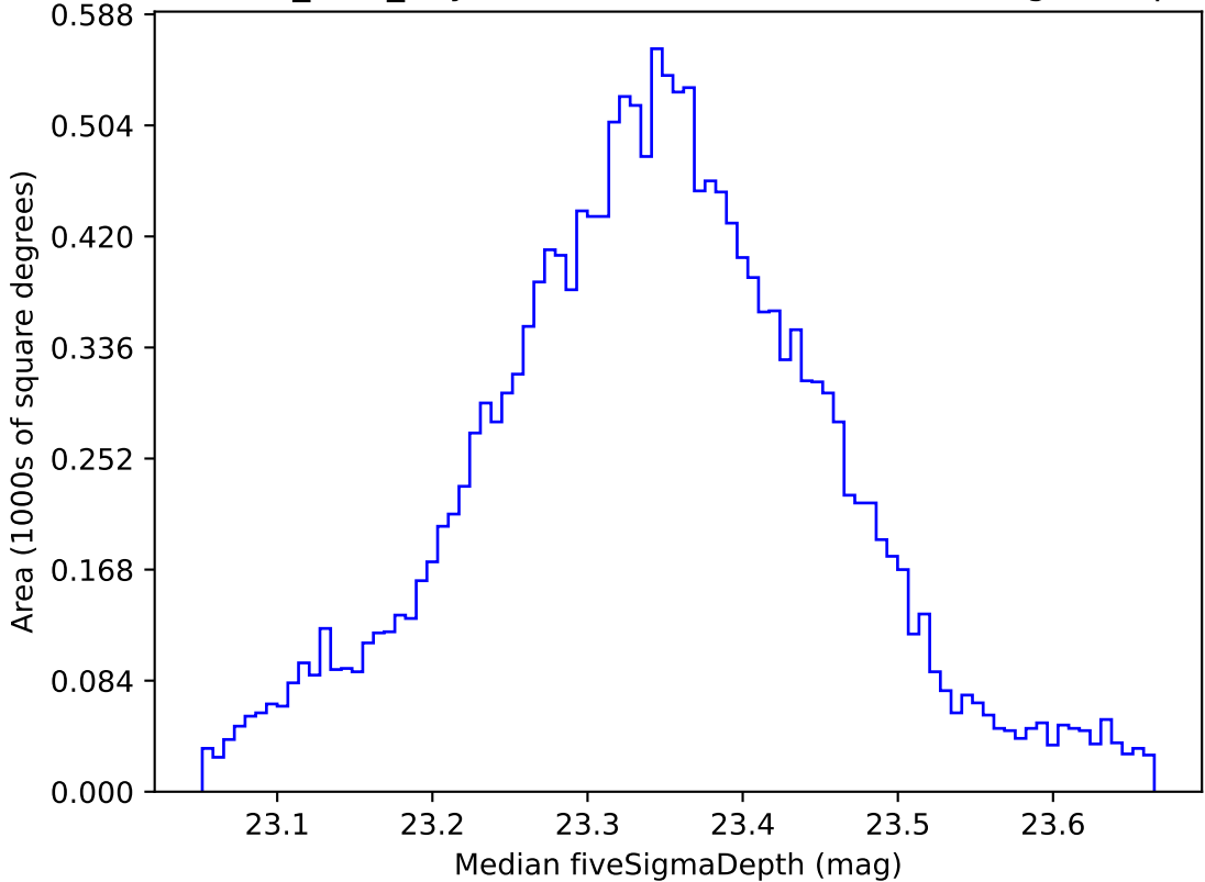
baseline_v3.5_10yrs WFD all bands: Median fiveSigmaDepth
