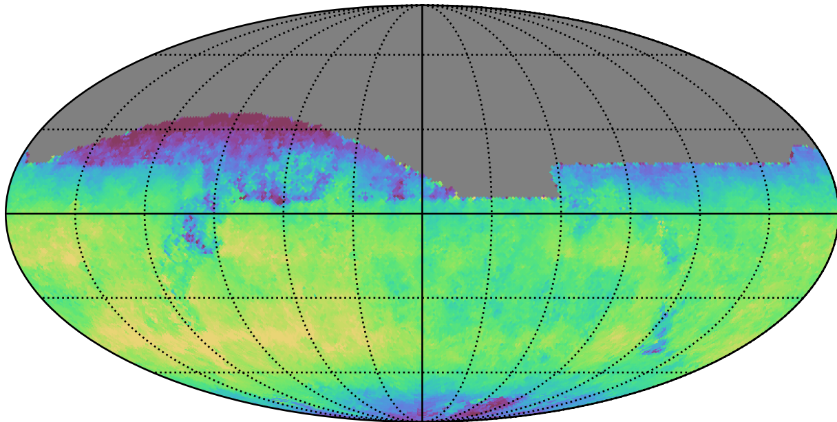
baseline_v3.5_10yrs All sky z band: Median fiveSigmaDepth
