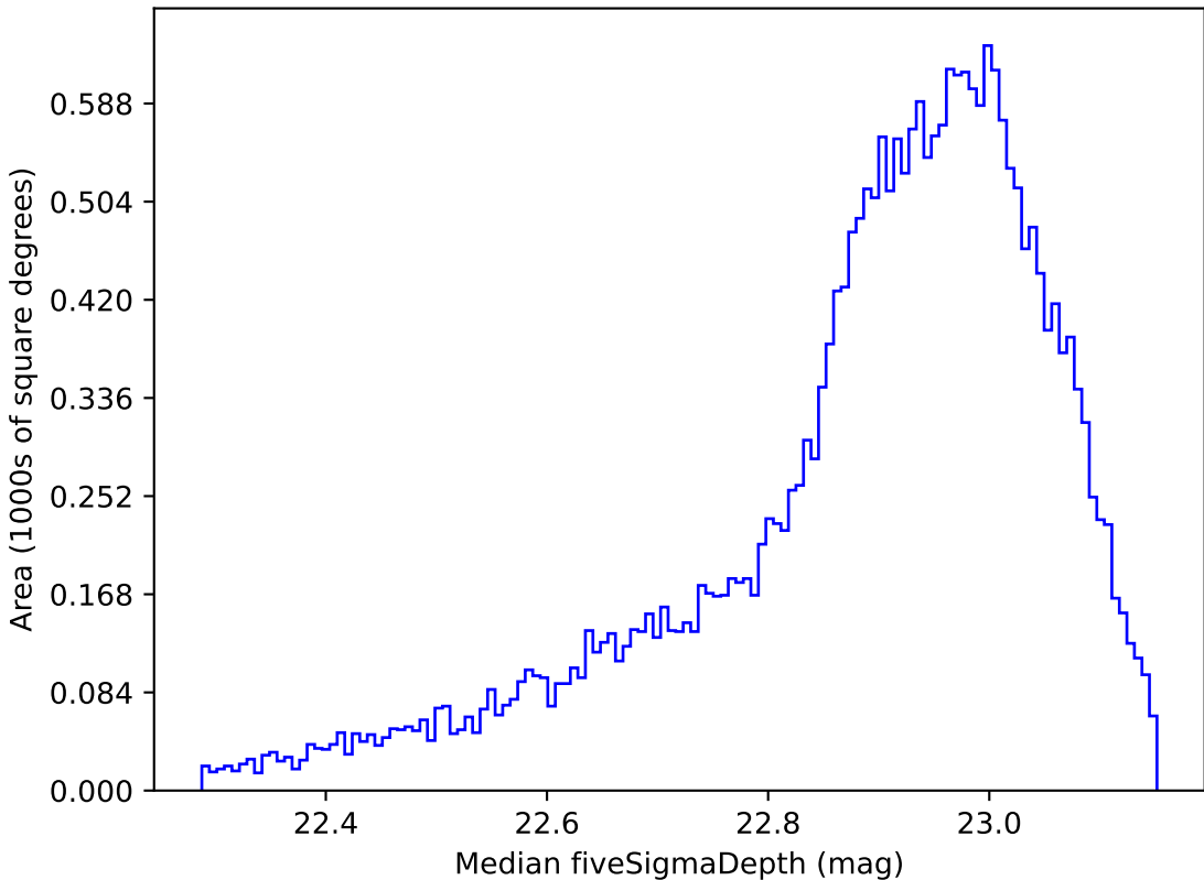
baseline_v3.5_10yrs All sky z band: Median fiveSigmaDepth
