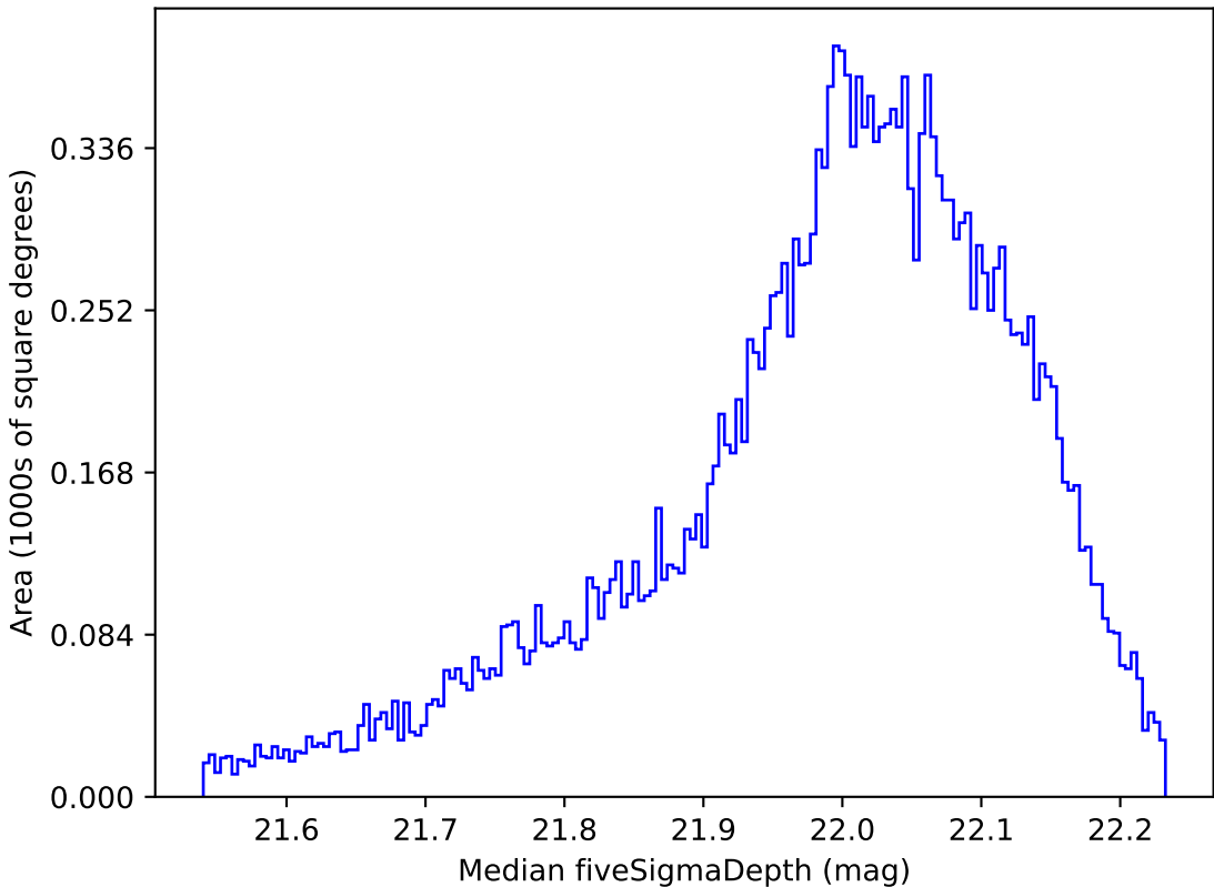
baseline_v3.5_10yrs All sky y band: Median fiveSigmaDepth
