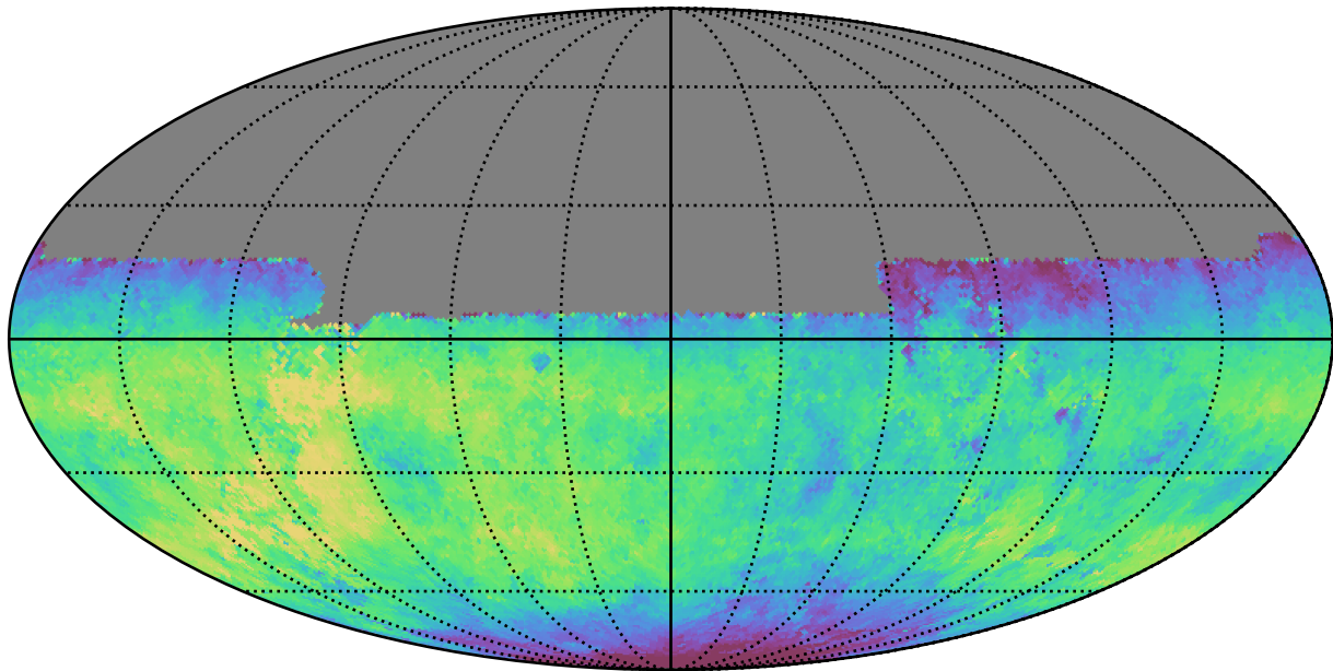
baseline_v3.5_10yrs All sky u band: Median fiveSigmaDepth
