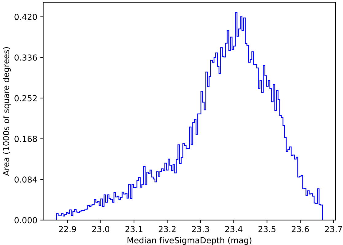
baseline_v3.5_10yrs All sky u band: Median fiveSigmaDepth
