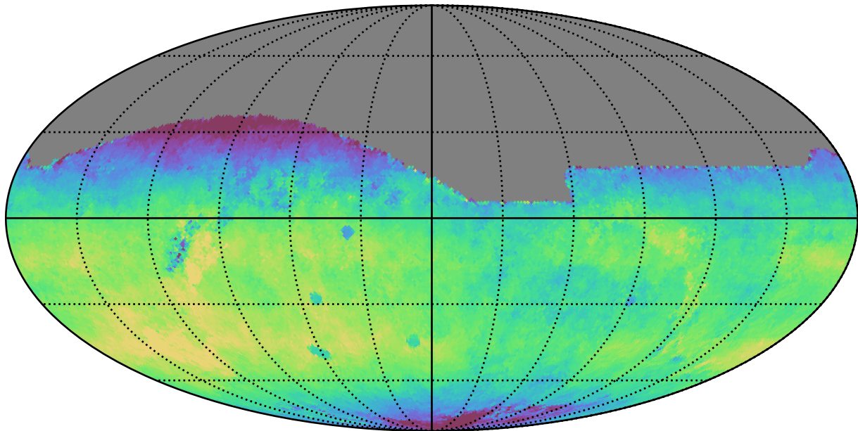
baseline_v3.5_10yrs All sky r band: Median fiveSigmaDepth
