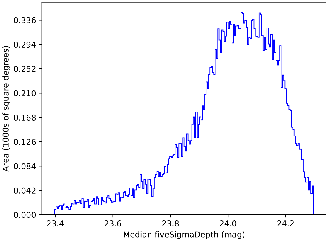
baseline_v3.5_10yrs All sky r band: Median fiveSigmaDepth
