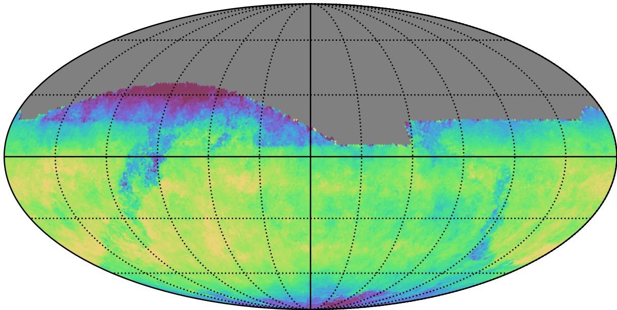
baseline_v3.5_10yrs All sky i band: Median fiveSigmaDepth
