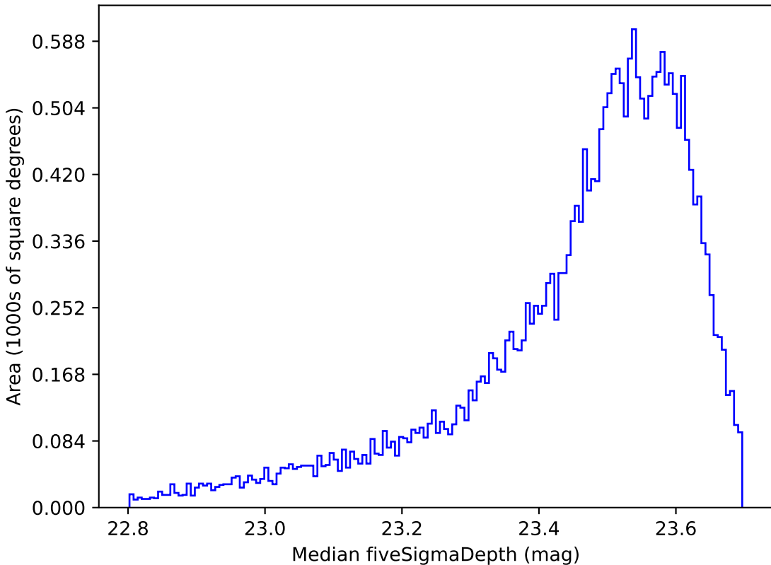
baseline_v3.5_10yrs All sky i band: Median fiveSigmaDepth
