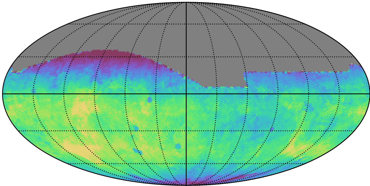
baseline_v3.5_10yrs All sky g band: Median fiveSigmaDepth
