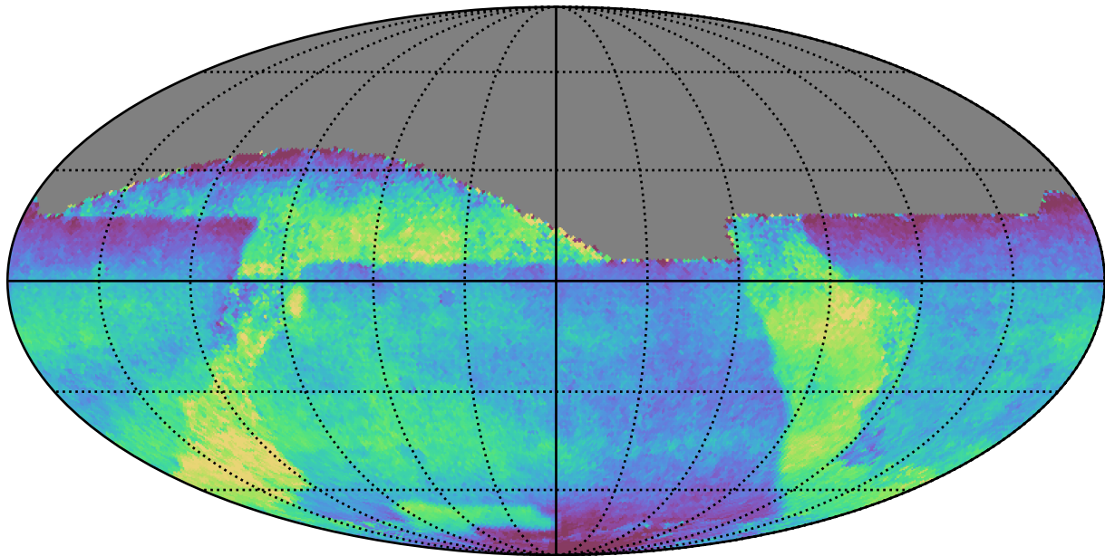
baseline_v3.5_10yrs All sky all bands: Median fiveSigmaDepth
