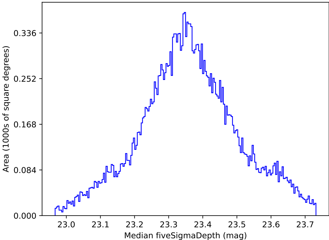
baseline_v3.5_10yrs All sky all bands: Median fiveSigmaDepth
