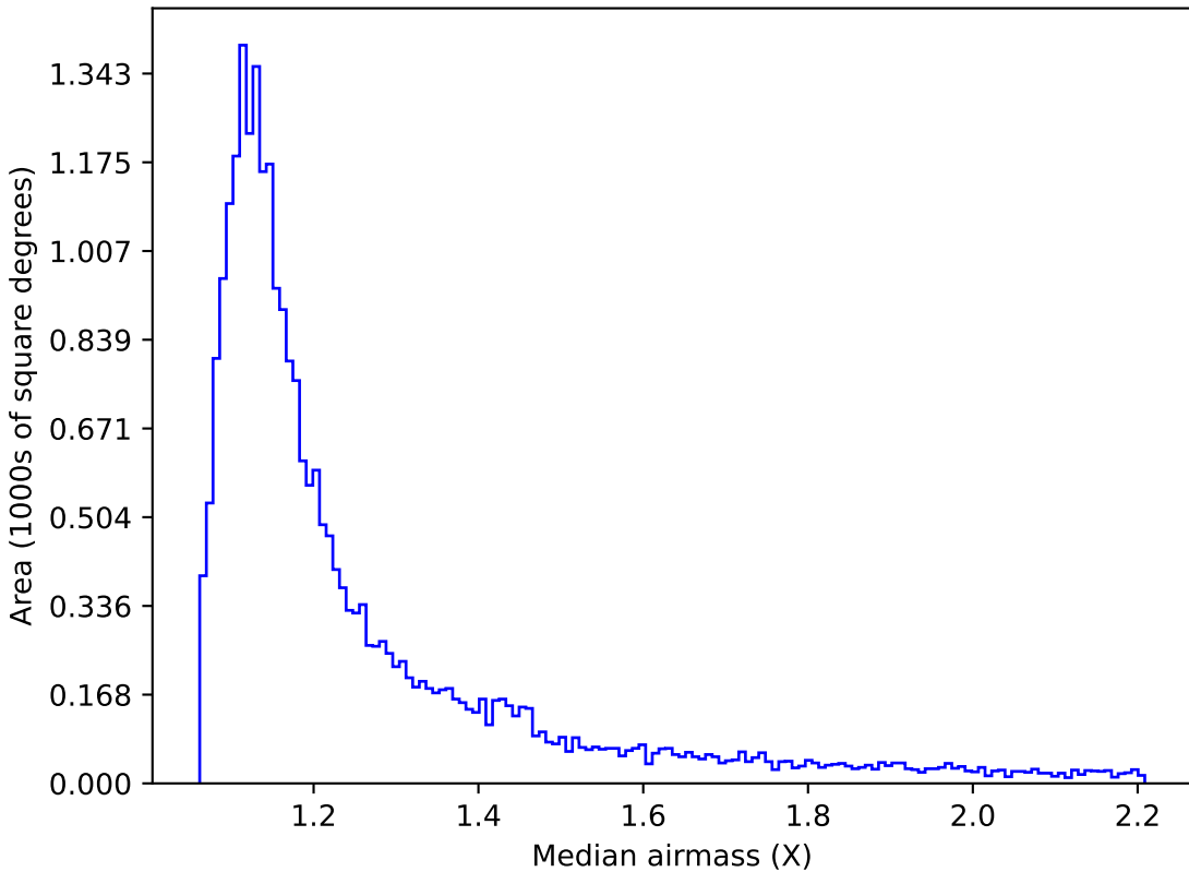
baseline_v3.5_10yrs Yr 1 z band: Median airmass
