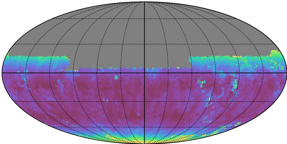
baseline_v3.5_10yrs Yr 1 y band: Median airmass
