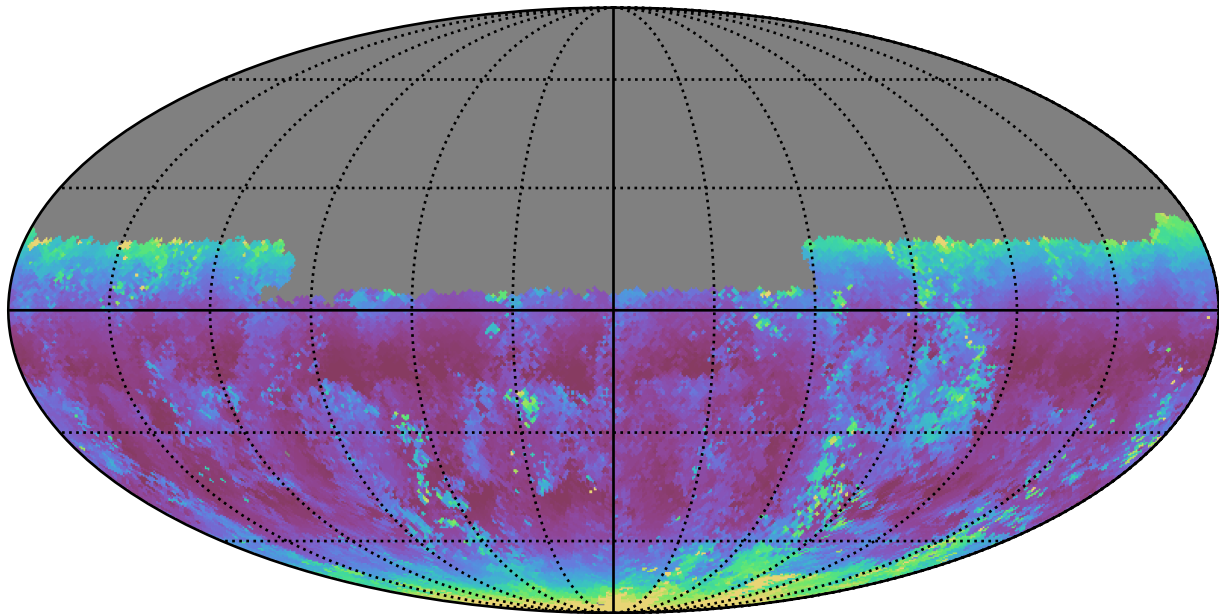
baseline_v3.5_10yrs Yr 1 u band: Median airmass
