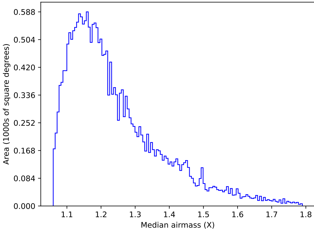
baseline_v3.5_10yrs Yr 1 u band: Median airmass
