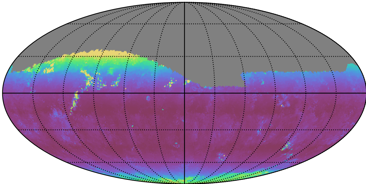
baseline_v3.5_10yrs Yr 1 i band: Median airmass
