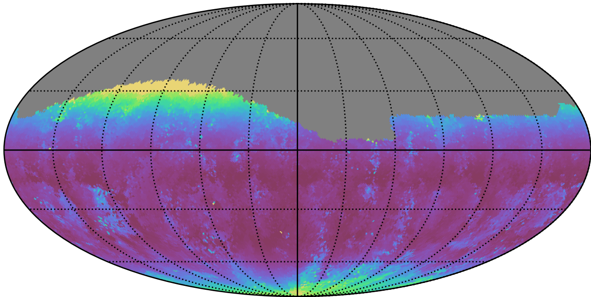
baseline_v3.5_10yrs Yr 1 g band: Median airmass
