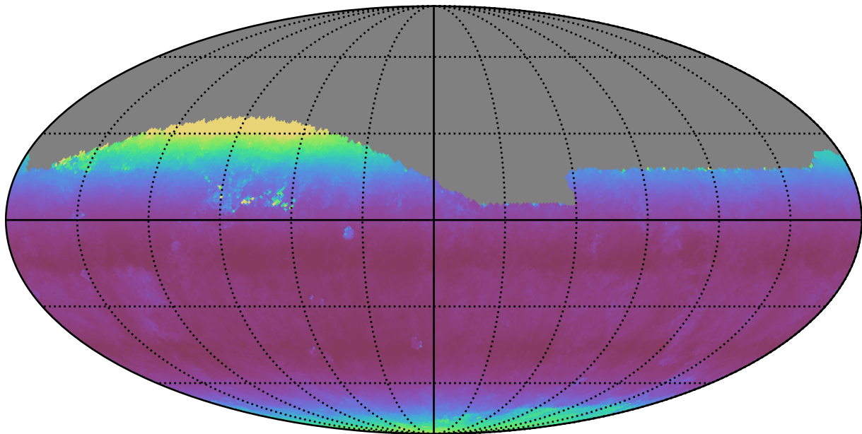
baseline_v3.5_10yrs Yr 1 all bands: Median airmass
