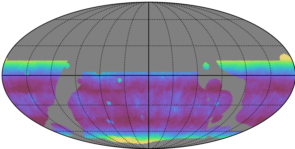
baseline_v3.5_10yrs WFD z band: Median airmass
