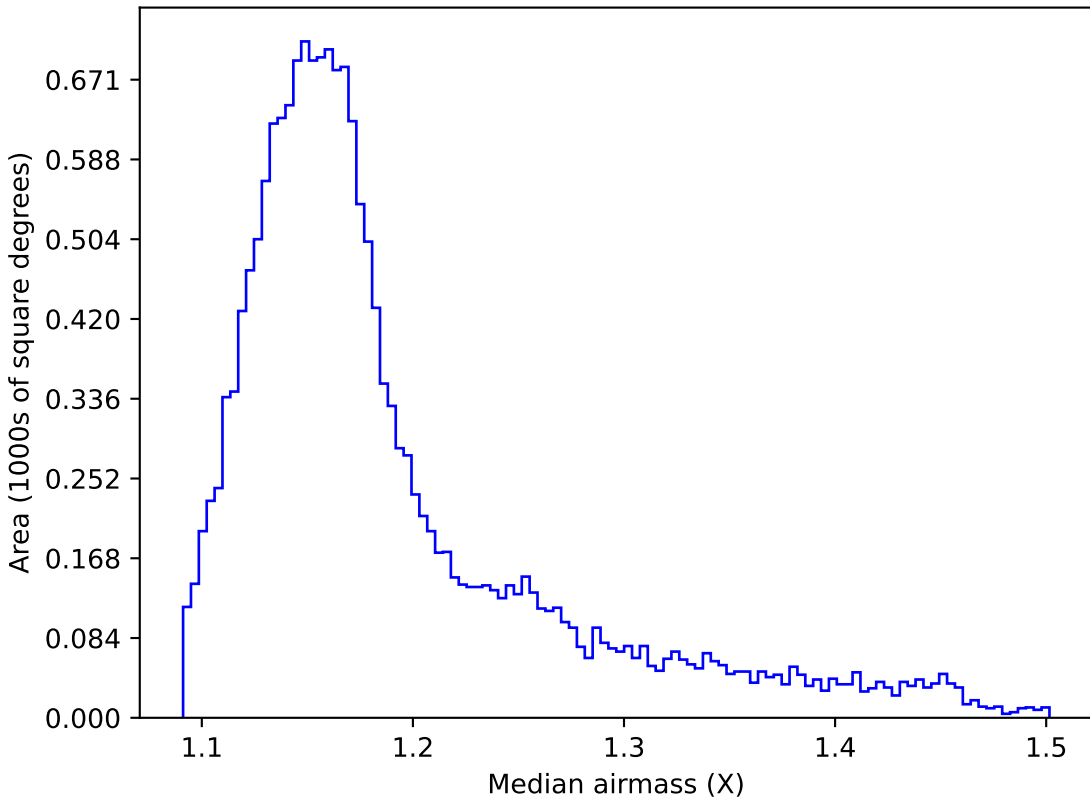
baseline_v3.5_10yrs WFD z band: Median airmass
