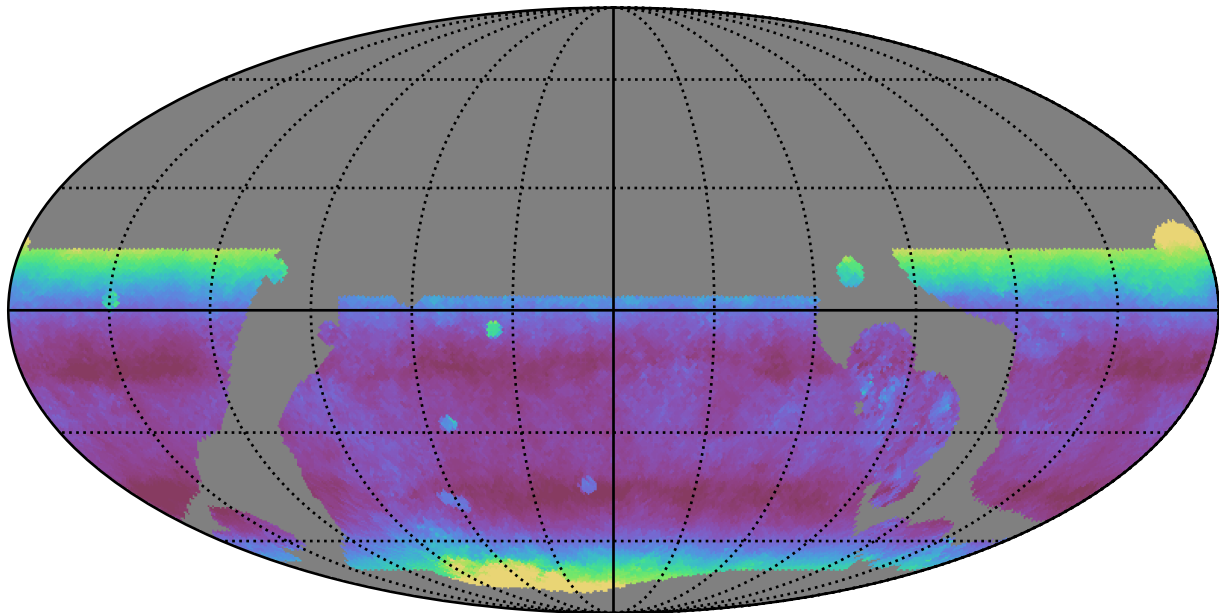
baseline_v3.5_10yrs WFD y band: Median airmass
