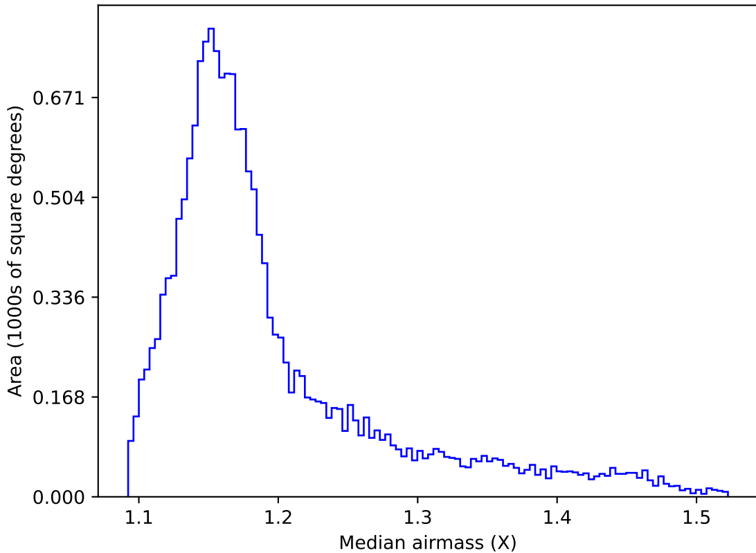
baseline_v3.5_10yrs WFD y band: Median airmass
