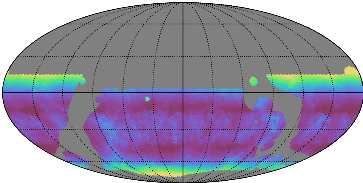
baseline_v3.5_10yrs WFD u band: Median airmass
