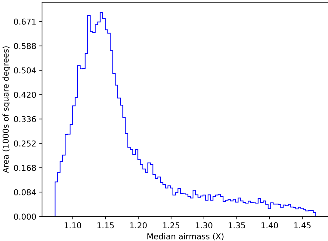
baseline_v3.5_10yrs WFD u band: Median airmass
