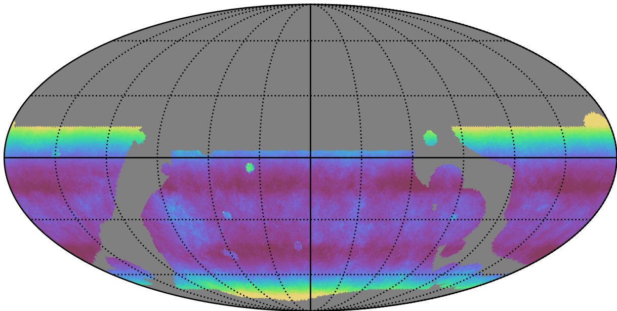
baseline_v3.5_10yrs WFD r band: Median airmass
