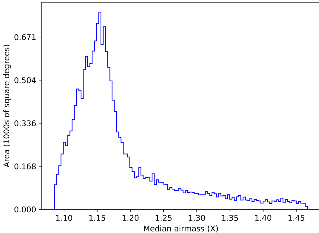
baseline_v3.5_10yrs WFD r band: Median airmass
