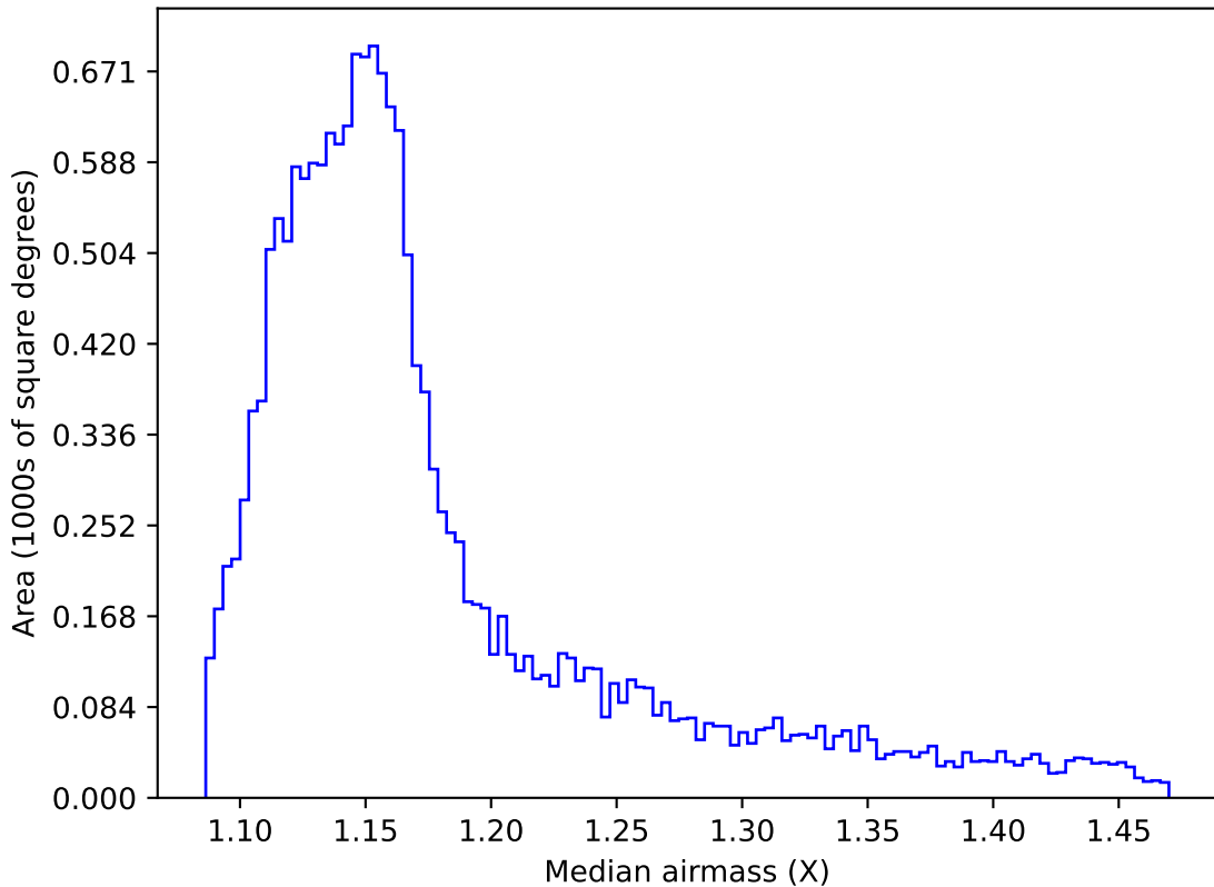
baseline_v3.5_10yrs WFD i band: Median airmass
