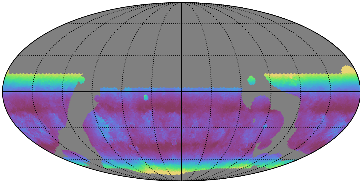
baseline_v3.5_10yrs WFD g band: Median airmass
