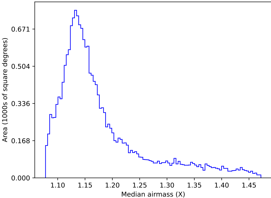
baseline_v3.5_10yrs WFD g band: Median airmass
